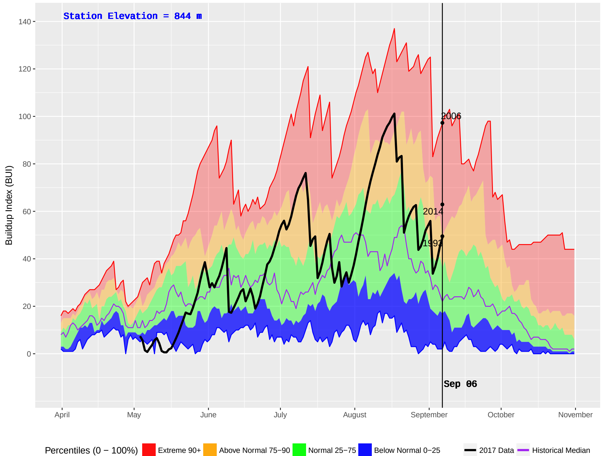
GANOKWA (182) : Historical (1993–2016) and Current (2017) Noon Buildup Index (BUI)
