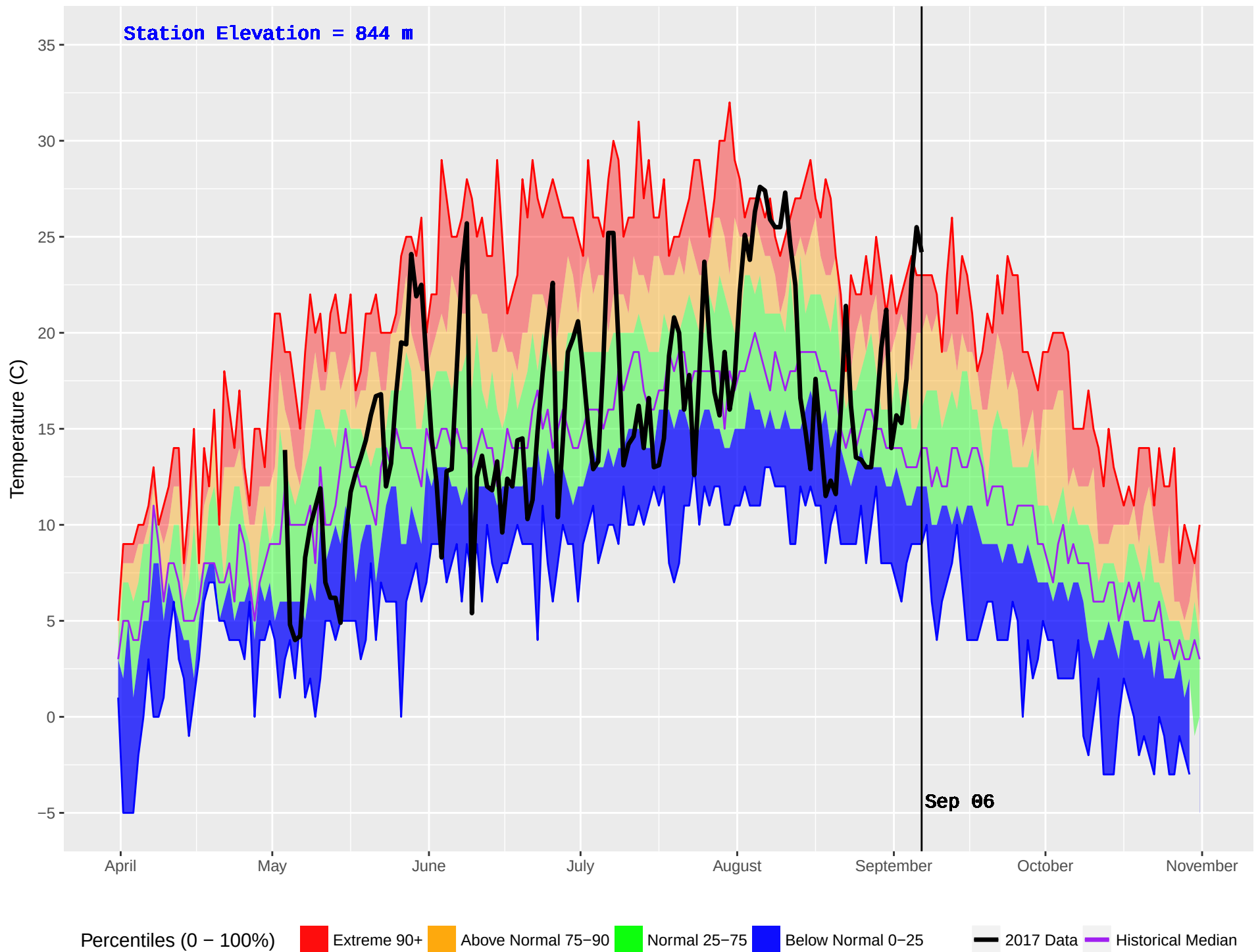
GANOKWA (182) : Historical (1993–2016) and Current (2017) Noon Temperature
