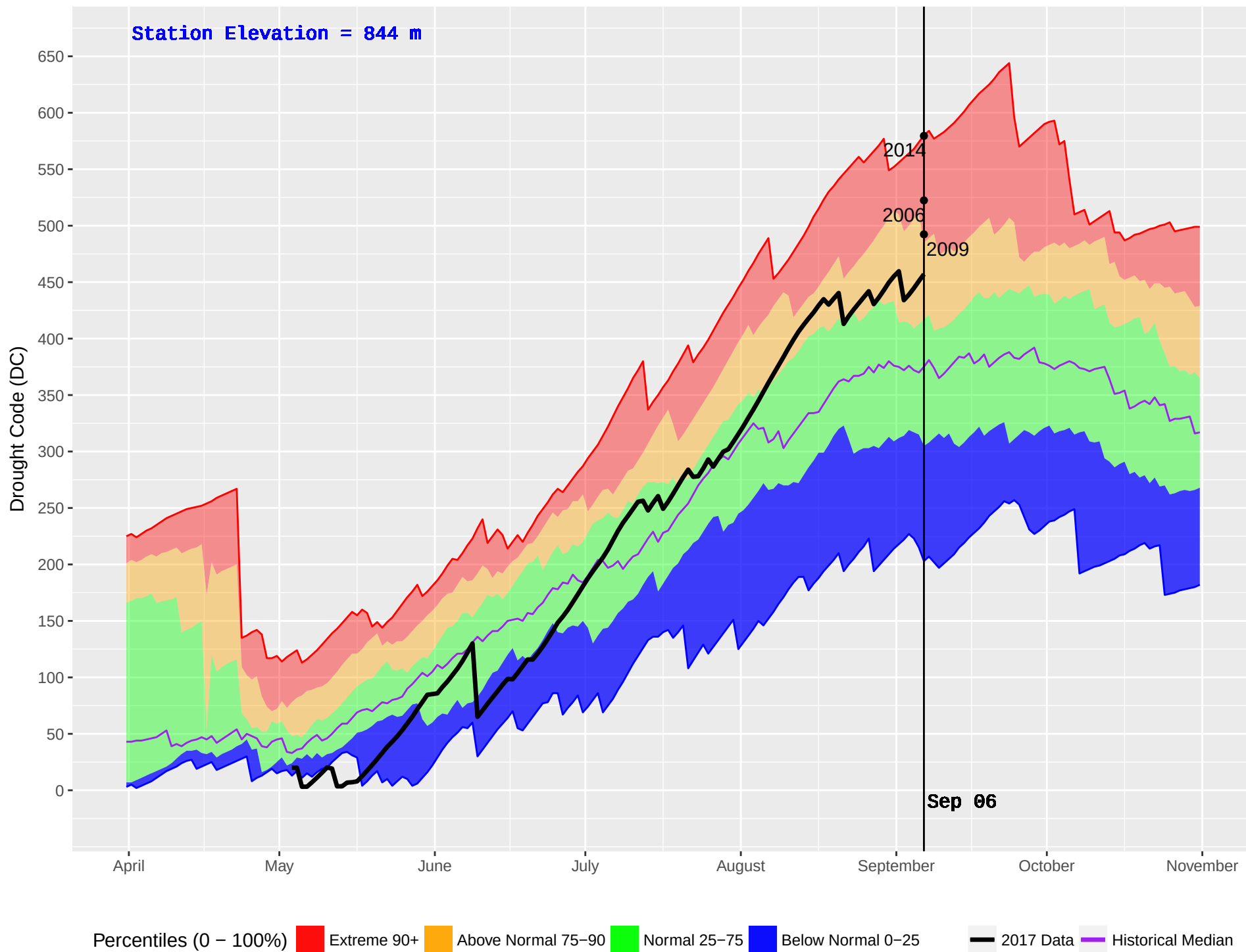
GANOKWA (182) : Historical (1993–2016) and Current (2017) Noon Drought Code (DC)
